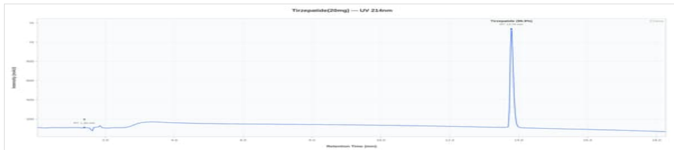
Tirzepatide 20mg - 2026-002: UV Chromatogram
