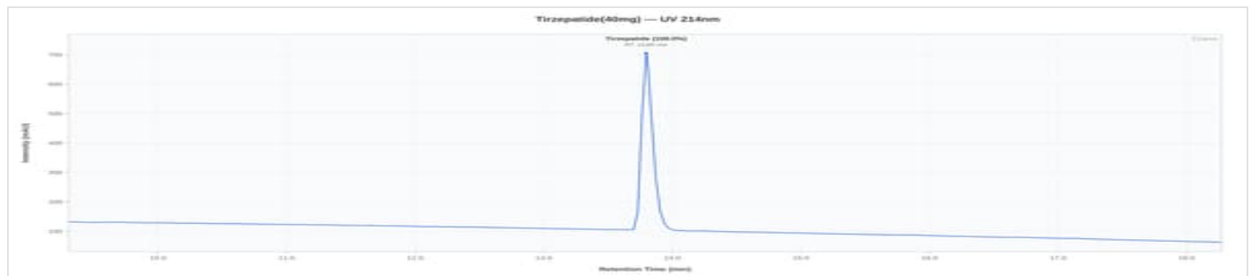
Tirzepatide 40mg - 2026-002: UV Chromatogram
