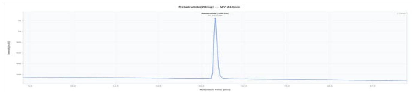
Retatrutide 20mg - 2026-002: UV Chromatogram
