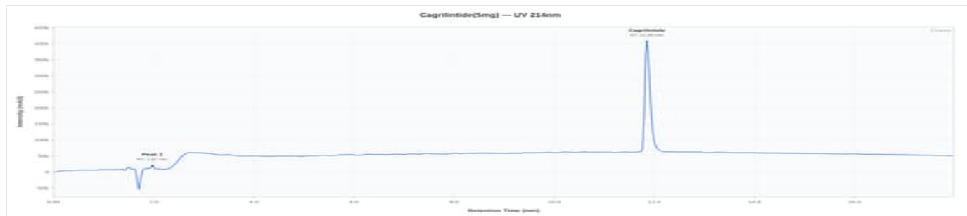
Cagrilintide 5mg - 2026-003: UV Chromatogram
