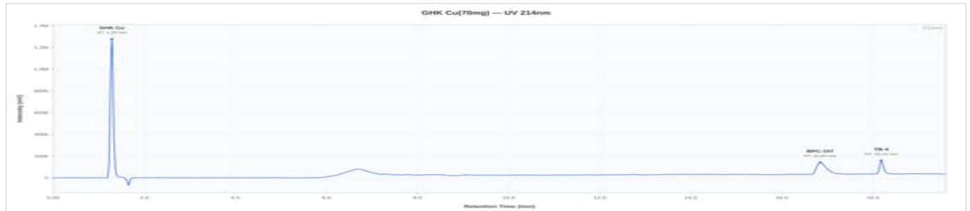
GLOW 70mg - 2026-003: UV Chromatogram
